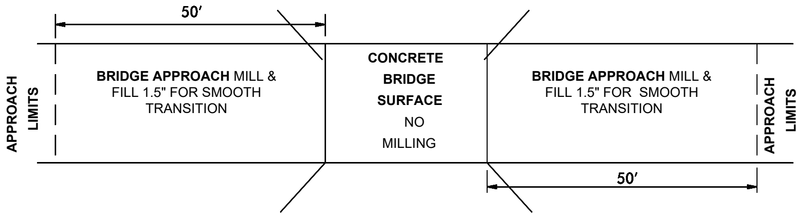
DETAIL FOR MAP # 2 & 3 / STRUCTURE # # 0086 & # 0207
