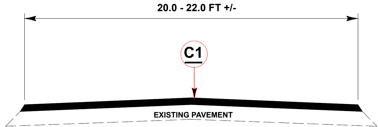
TYPICAL SECTION # 1 MAP(S) # 1, 3, 6, & 8 - 13
