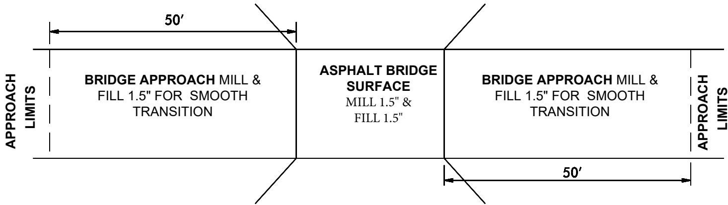
DETAIL FOR MAP # 1 & 8 / STRUCTURE # 00236 & 0003
